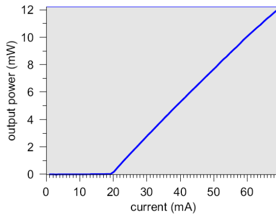
Power against Operating Current
